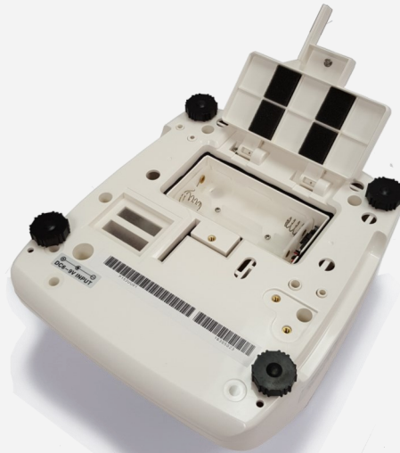
DS-500 Scale Battery Opening For 4 C Size Dry Batteries
